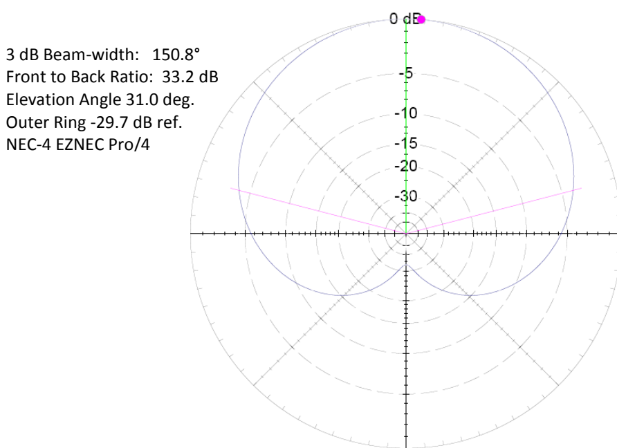
Figure 14. Typical Antenna Pattern for a 34ft x 16ft FLAG @ 10ft (1.9 MHz)
