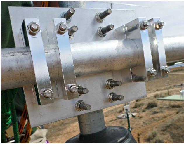
Boom to Mast Plate attached to Boom
